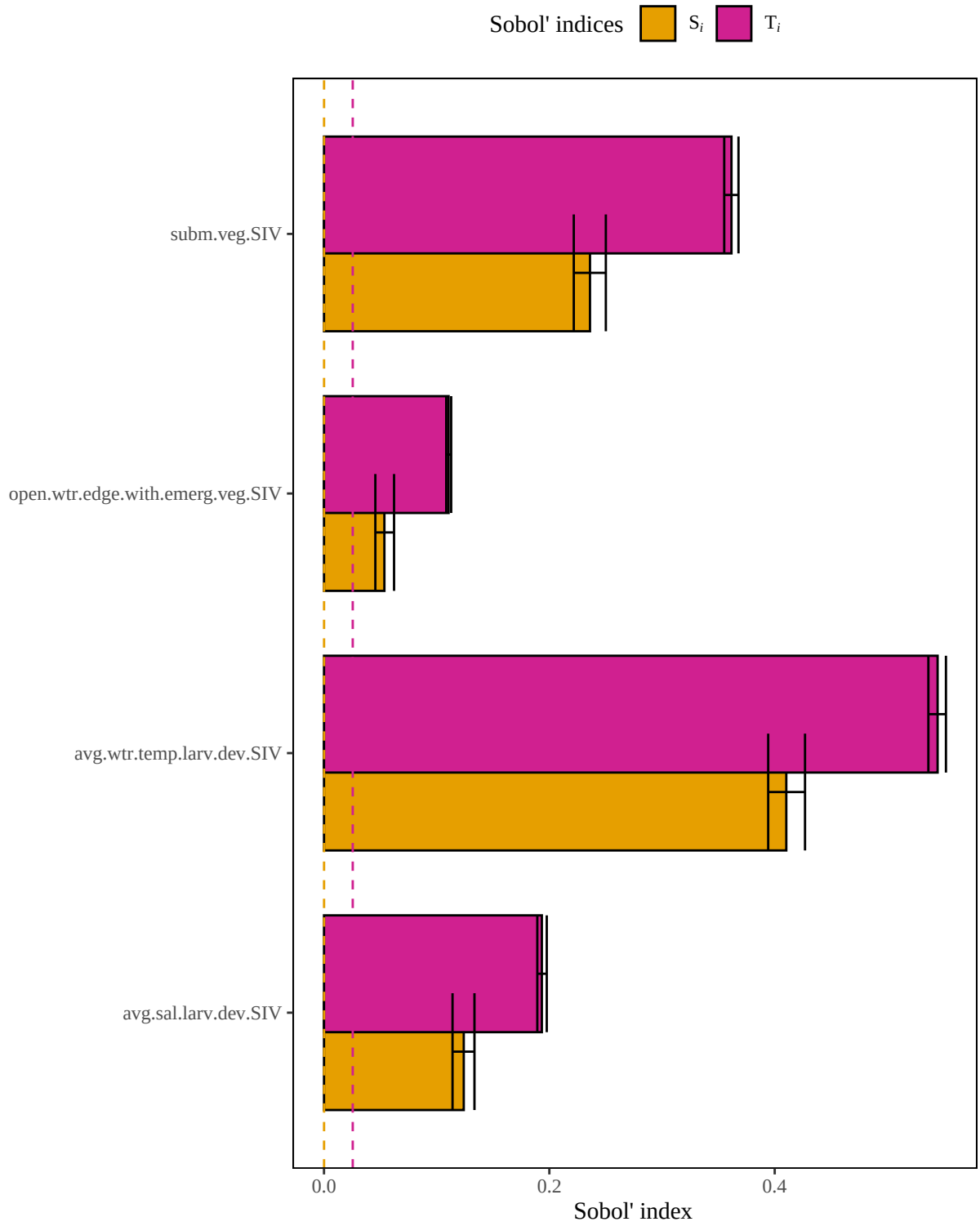
Figure 3. Results of a sensitivity analysis for the reddrumLarvJuvEstuSubmVeg model based on the original author-specified model outlined in Buckley (1984). Dashed lines represent baseline numerical approximation error for S_i and T_i ( i.e. , dummy variables).
